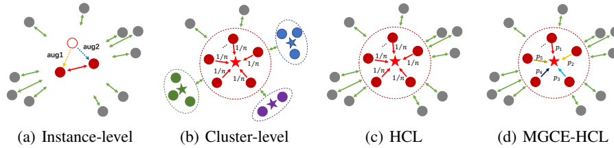
Fig. 1. Illustration for different contrastive learning paradigms. Red arrows in a), b) and c): pulling together; Green arrows: pushing away. (a) For instance-level paradigm, two augmented samples (red points) of original input (red circle) are pulled together and push all others away. (b) For cluster-level paradigm, positive samples (red points) are pushed to the cluster center (red star), and different clusters are mutually exclusive. (c) In our HCL, different from (a) and (b), we consider all negative samples (grey points) individually as individual class. (d) In MGCE-HCL, we further use the priority to weight the similarity between positive samples.
