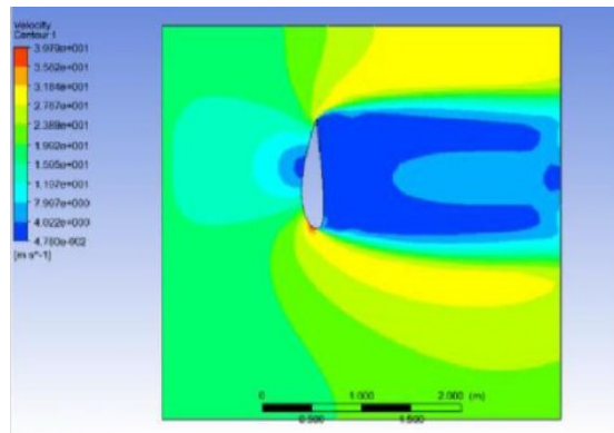
Fig .5. Velocity plot -450 blade angle
