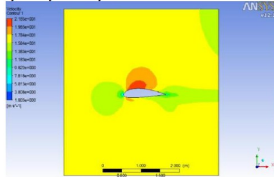
Fig 3. Velocity plot -00 blade angle
