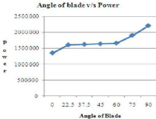
Fig 7.Effect of power in various angle of blade
