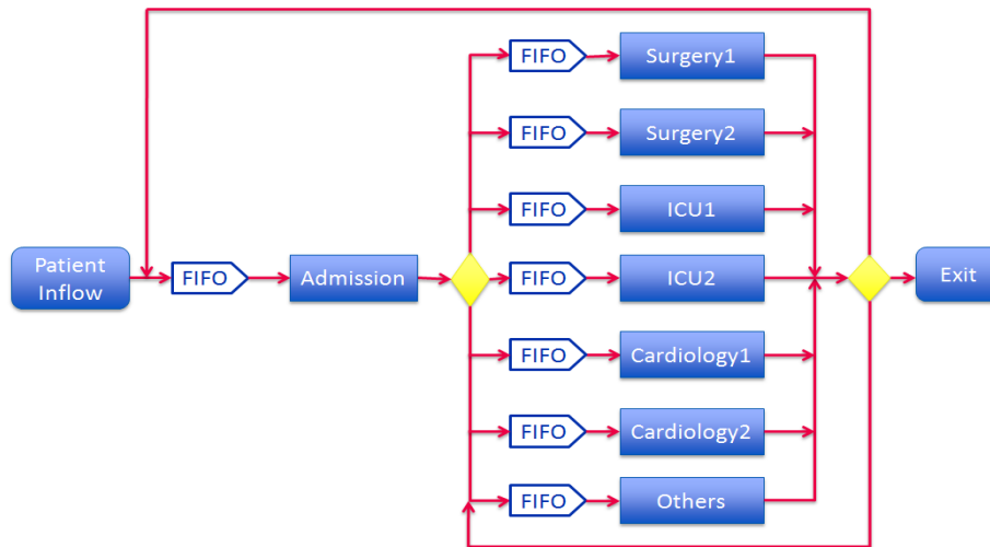
Fig. 2. The conceptual model of in-hospital patient flow simulation.
