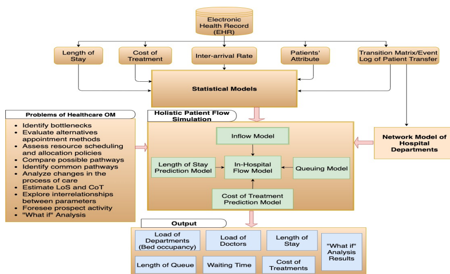
Fig. 1. The proposed model architecture.
