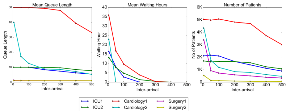
Fig. 7. Load of departments as the inter-arrival rate change (capacity of CD1 = 50).
